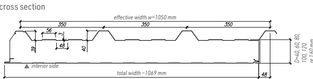
PIRTECH roof sandwich panels
