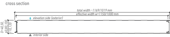
PIRTECH wall sandwich panel - standard
