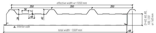
PIRTECH roof sandwich panels
