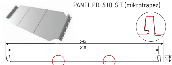
PANEL PD-510-S T (mikrotrapez)
